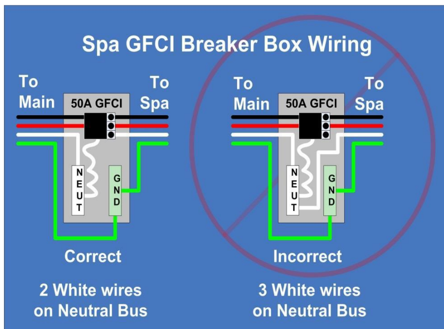
Figure 2 – GFCI Wiring
